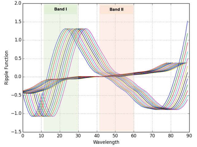
Fig. 4. Wavelength-dependent gain functions utilized for the simulation of detailed EDFA behaviour.
