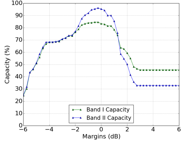
Fig. 5. Network capacity vs. OSNR margins applied by the control plane.
